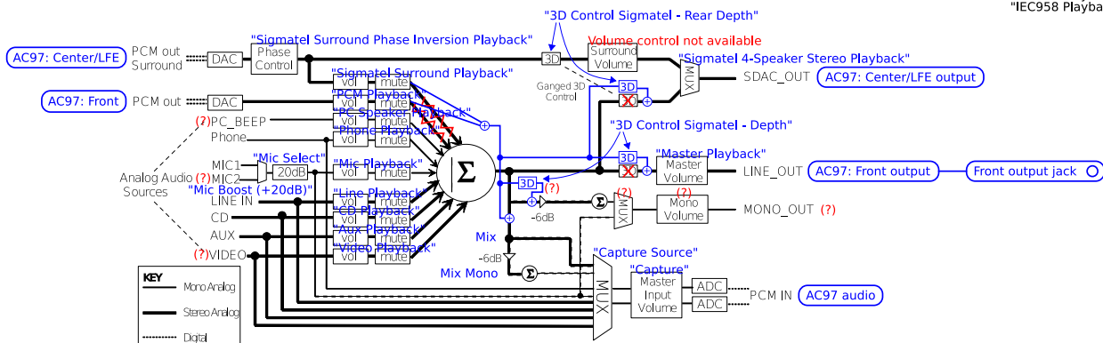
Figure 11. STAC9708/11 Mixer Functional Diagram
